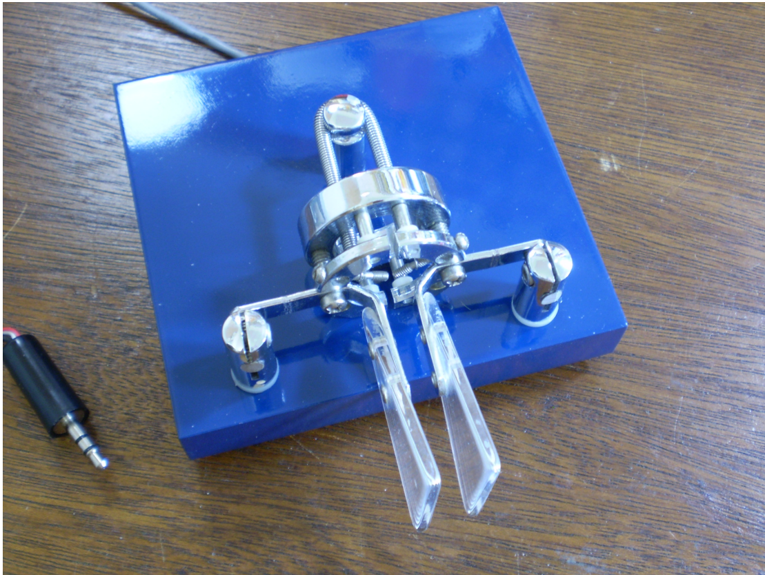
Figure 2: K7QO modifications to a Bencher BY-1.
