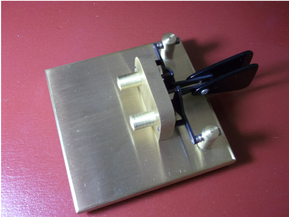
Figure 1: The prototype for the Vibroplex Brass Racer.
