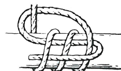
HALYARD BEND
