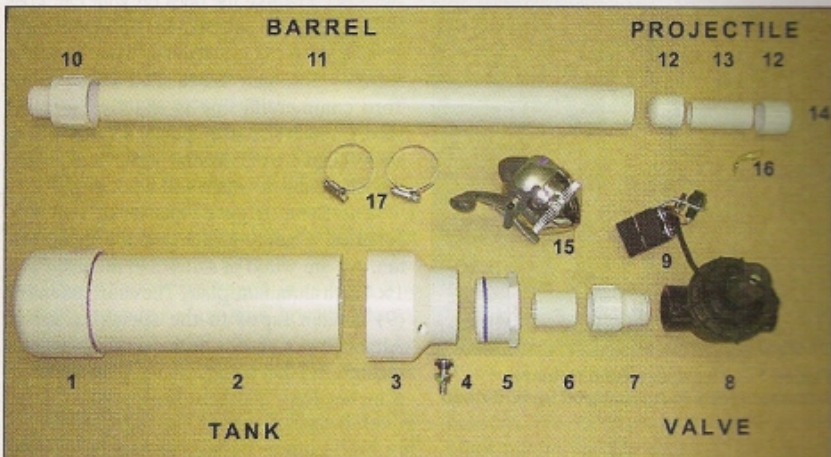
Figure 5 — Key parts of the spudgun.
