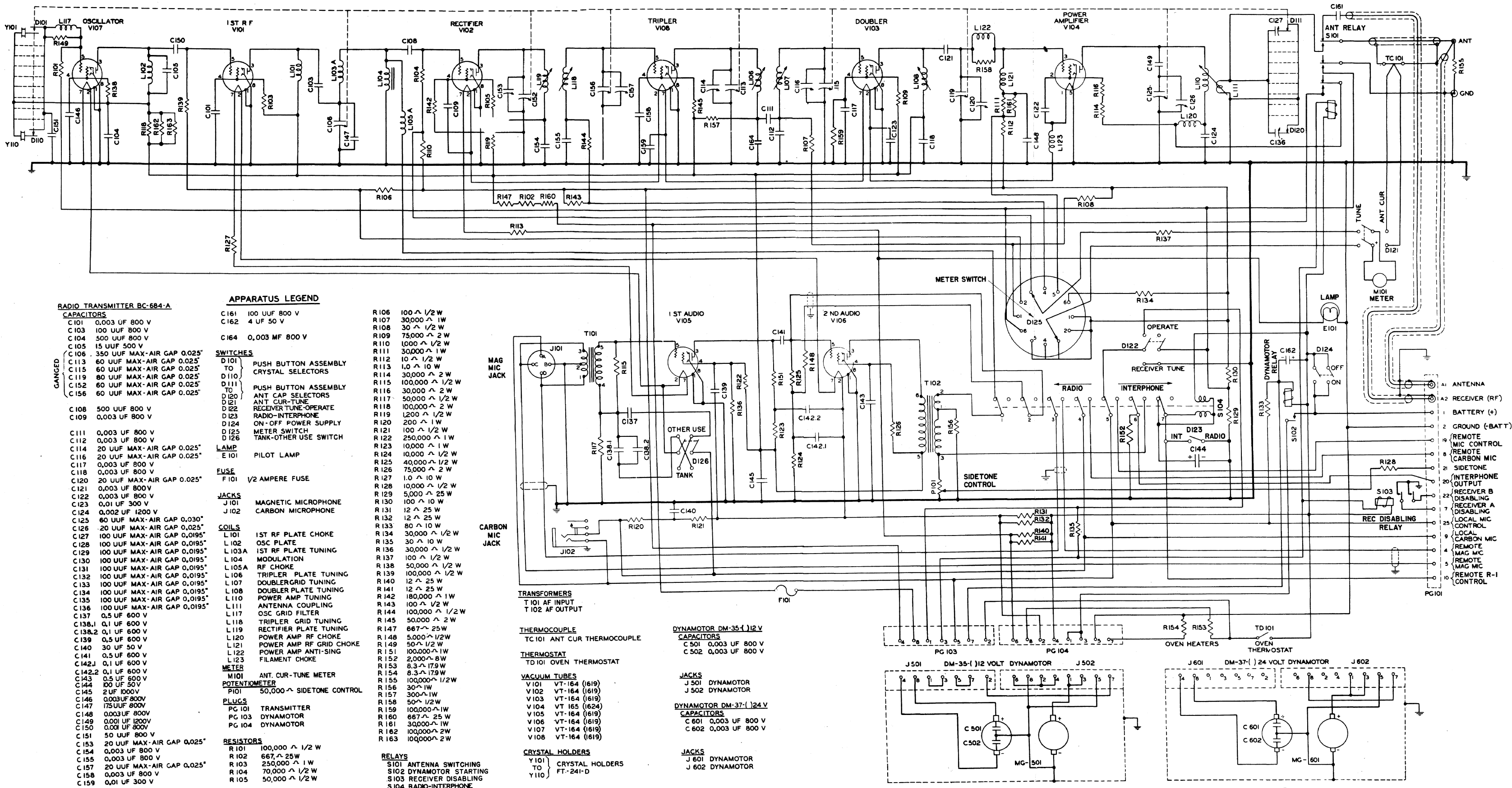
Fig. 74.1. Radio Transmitter BC-684-B: Schematic Diagram
