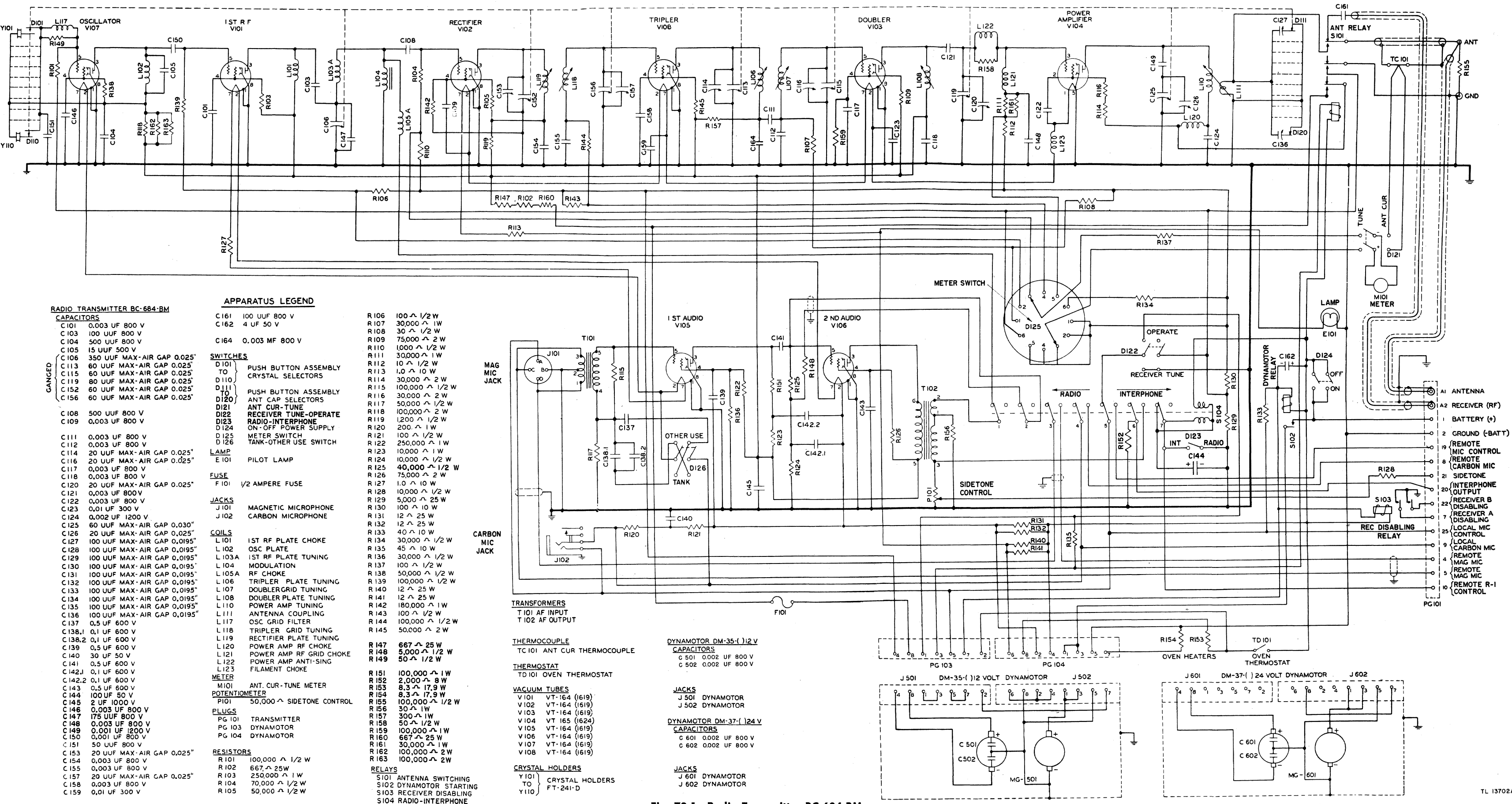
Fig. 73.1. Radio Transmitter BC-684-BM: Schematic Diagram
