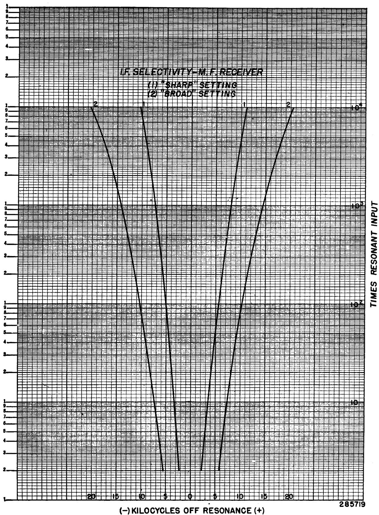
Figure 9-3—I.F. Selectivity—M.F. Receiver (Curve 285719)
