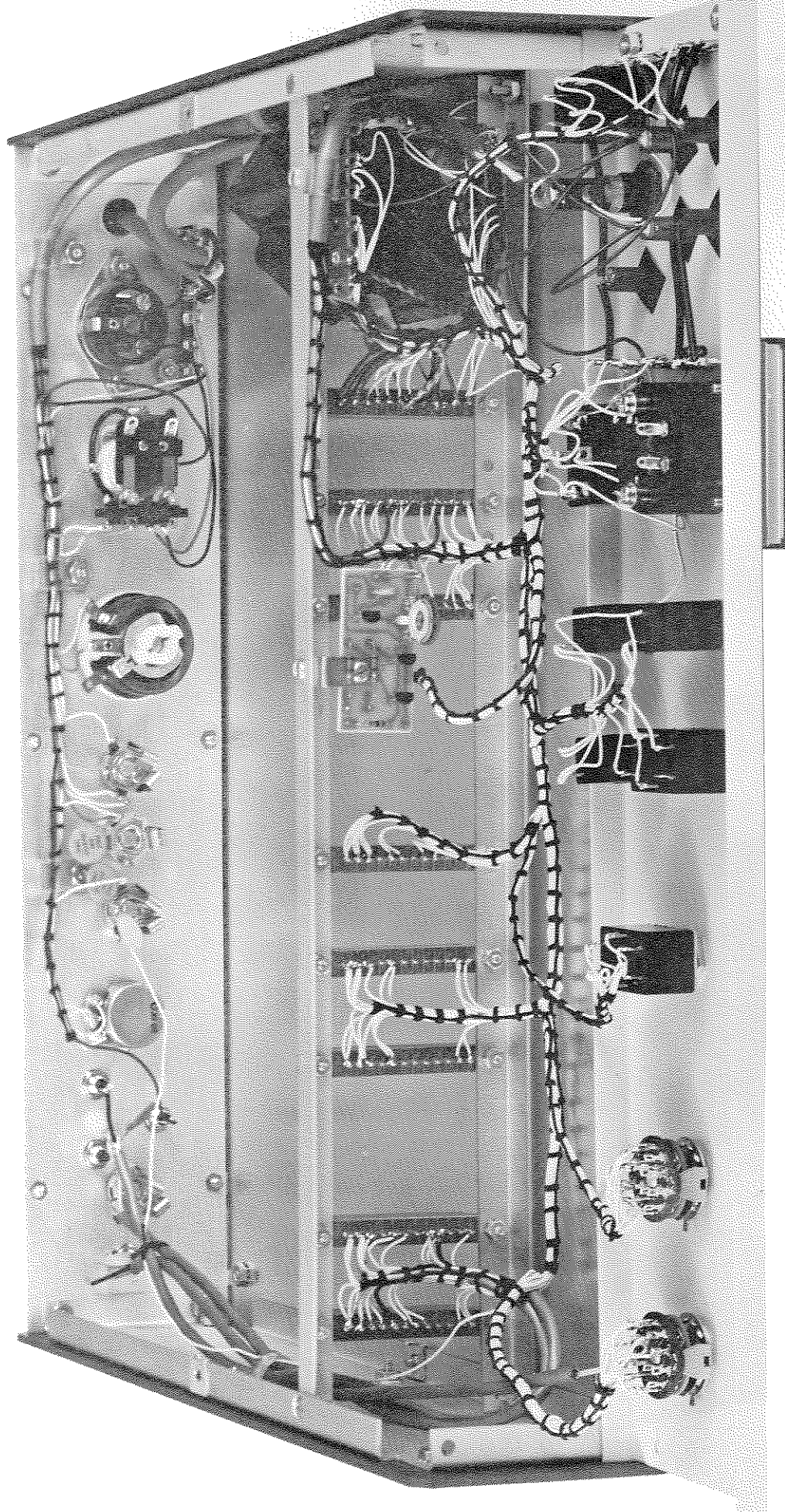
Figure 18 Cabinet Pictorial
