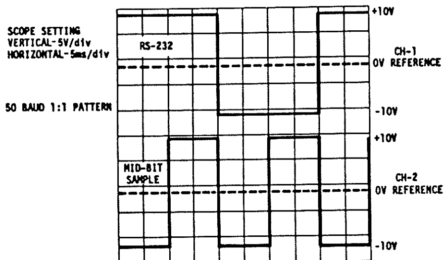
Figure 5-6. Mid-Bit Sample
