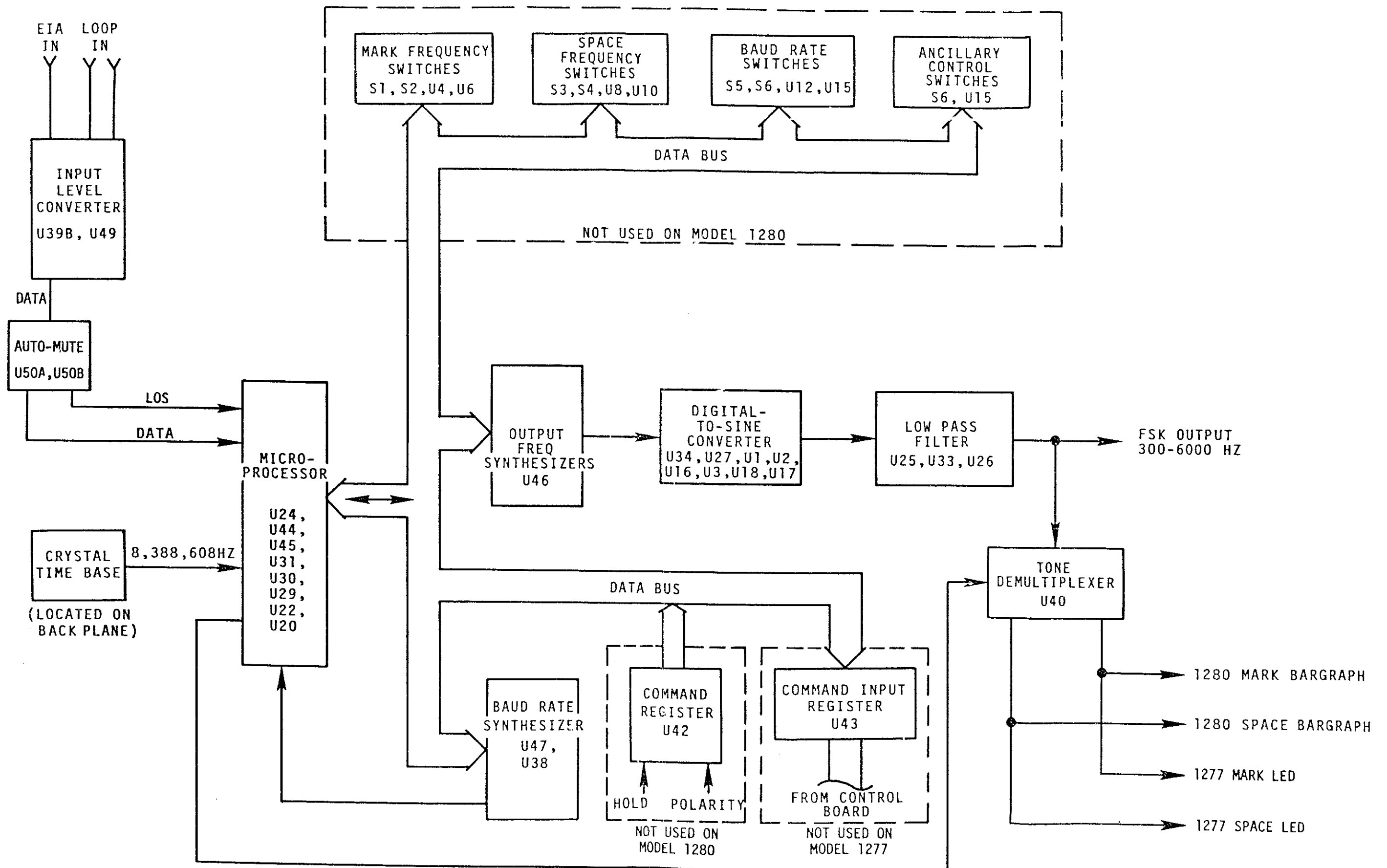
Figure 4-5. Modulator Block Diagram
