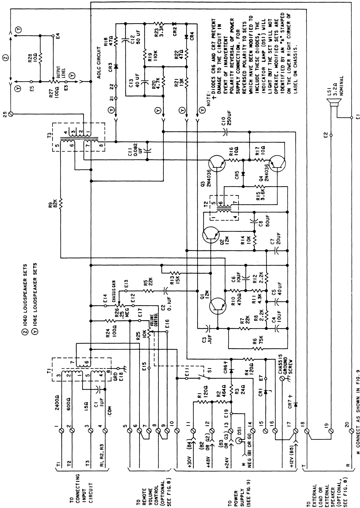
Fig. 13—Schematic—106D and E Loudspeaker Sets
