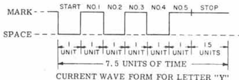
Figure 1 — Teletypewriter Code (5-Level)
