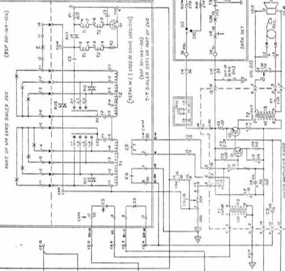
FS-9 TOUCH-TONE DIALER & AMPLIFIER
