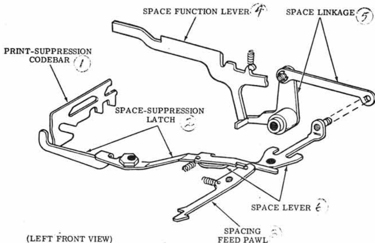
145 -- Space Function and Space-Suppression Mechanism
