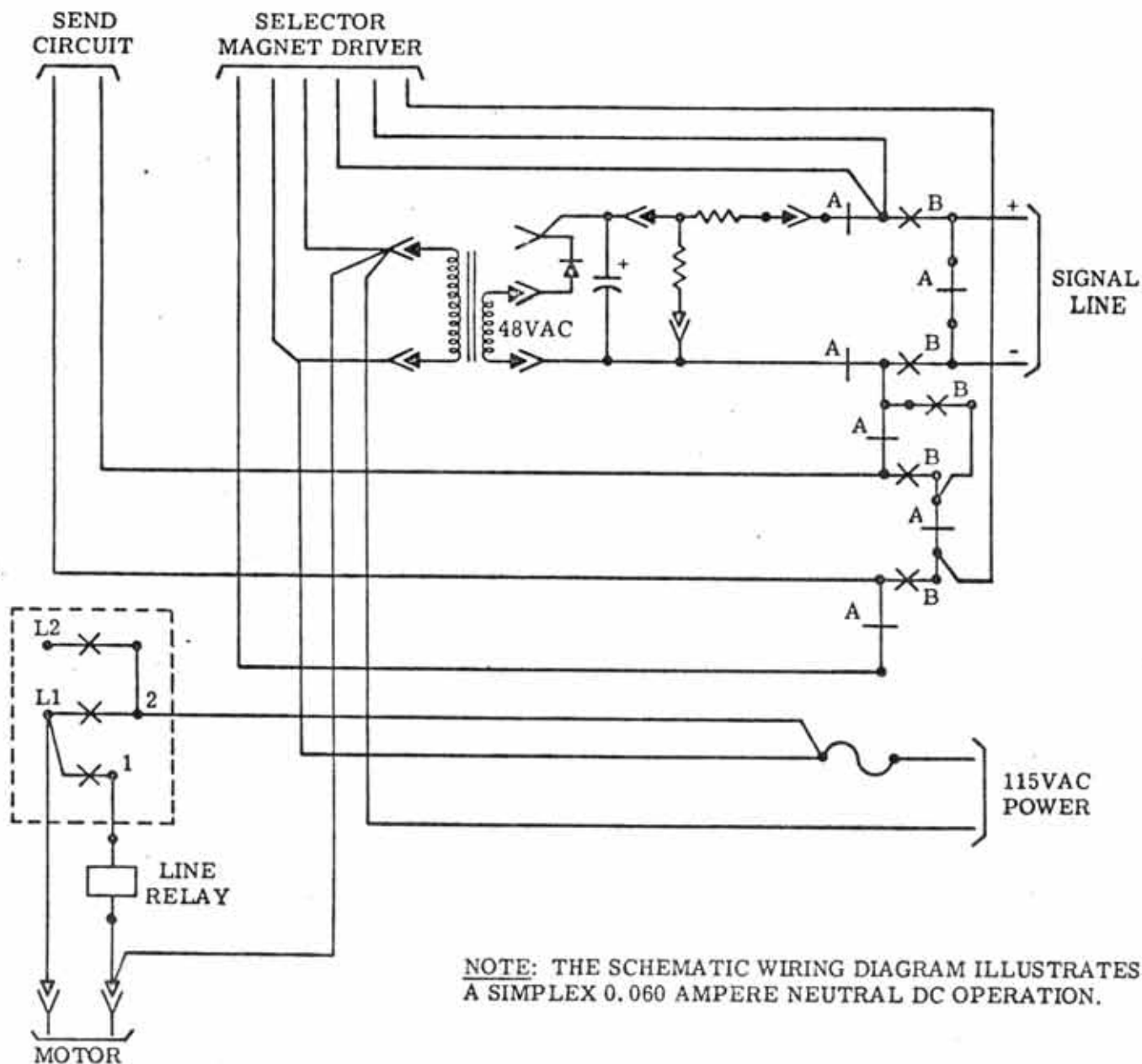
Figure 17 - Rotary Power Switch and Local Power Supply Circuit
