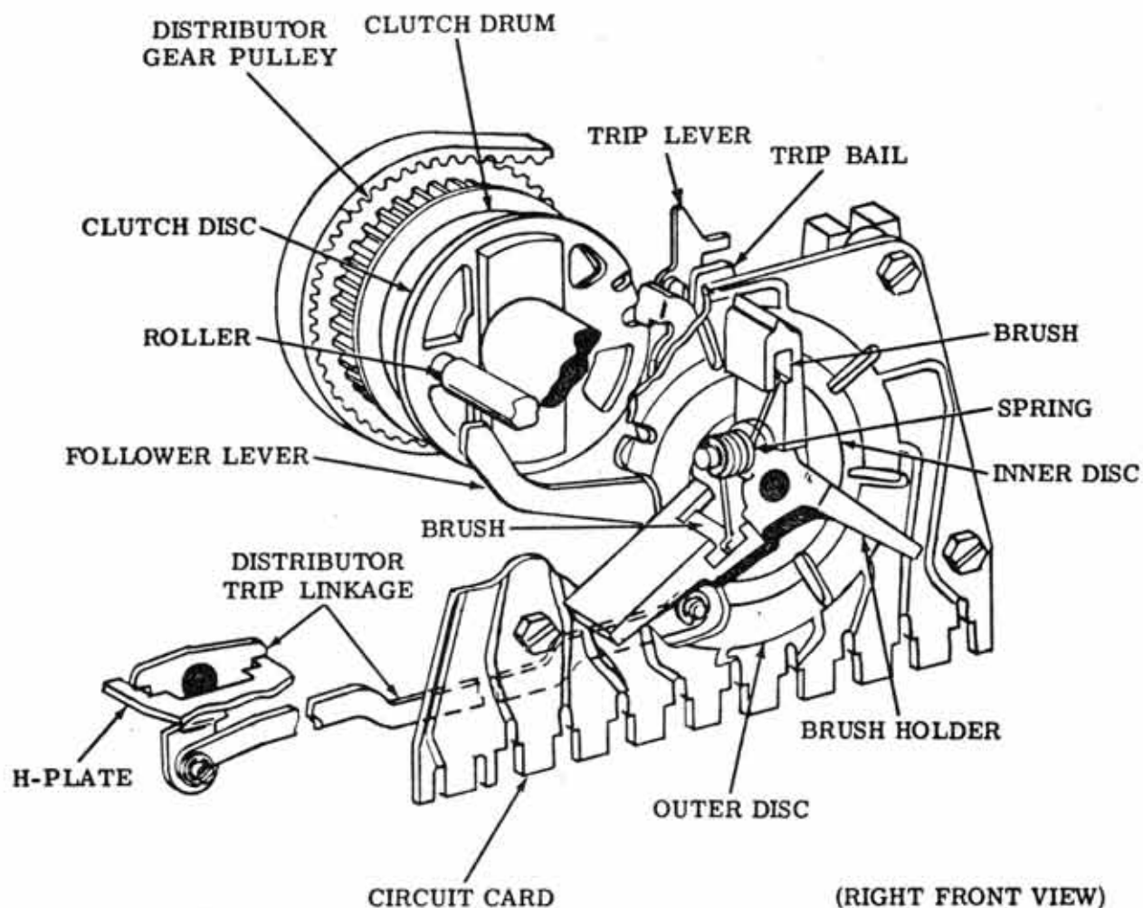
Distributor Mechanism
