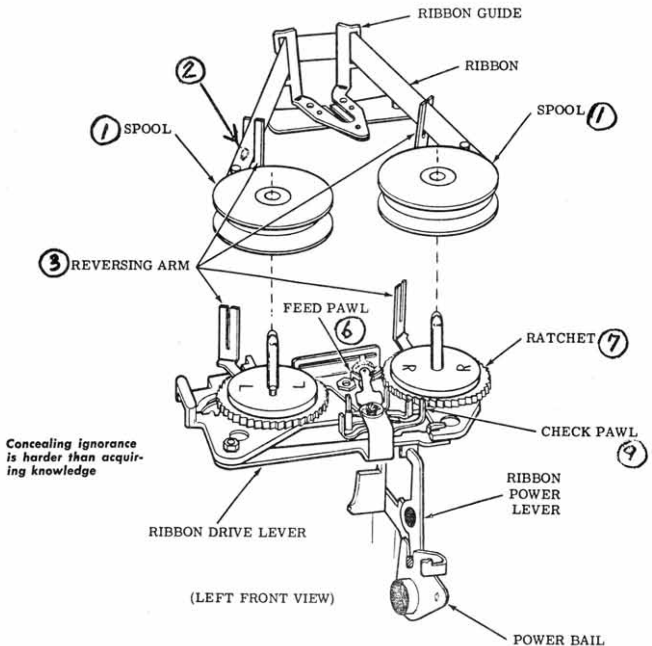
- Ribbon Mechanism
