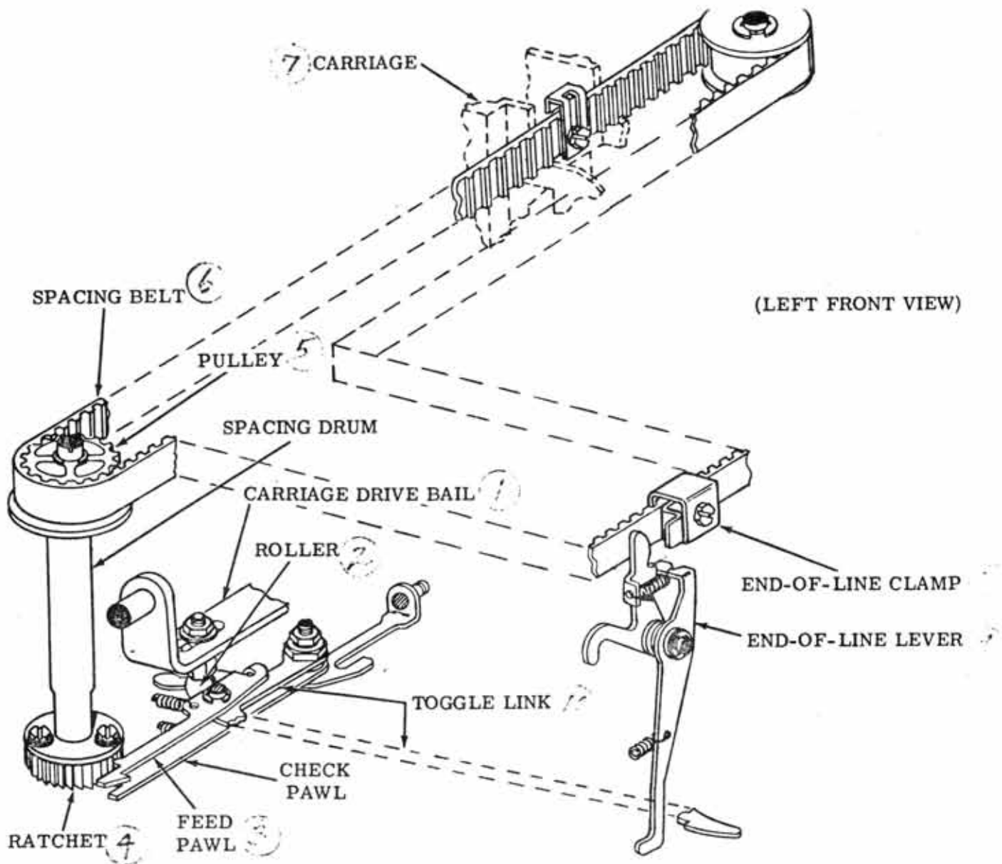
— Spacing Mechanism
