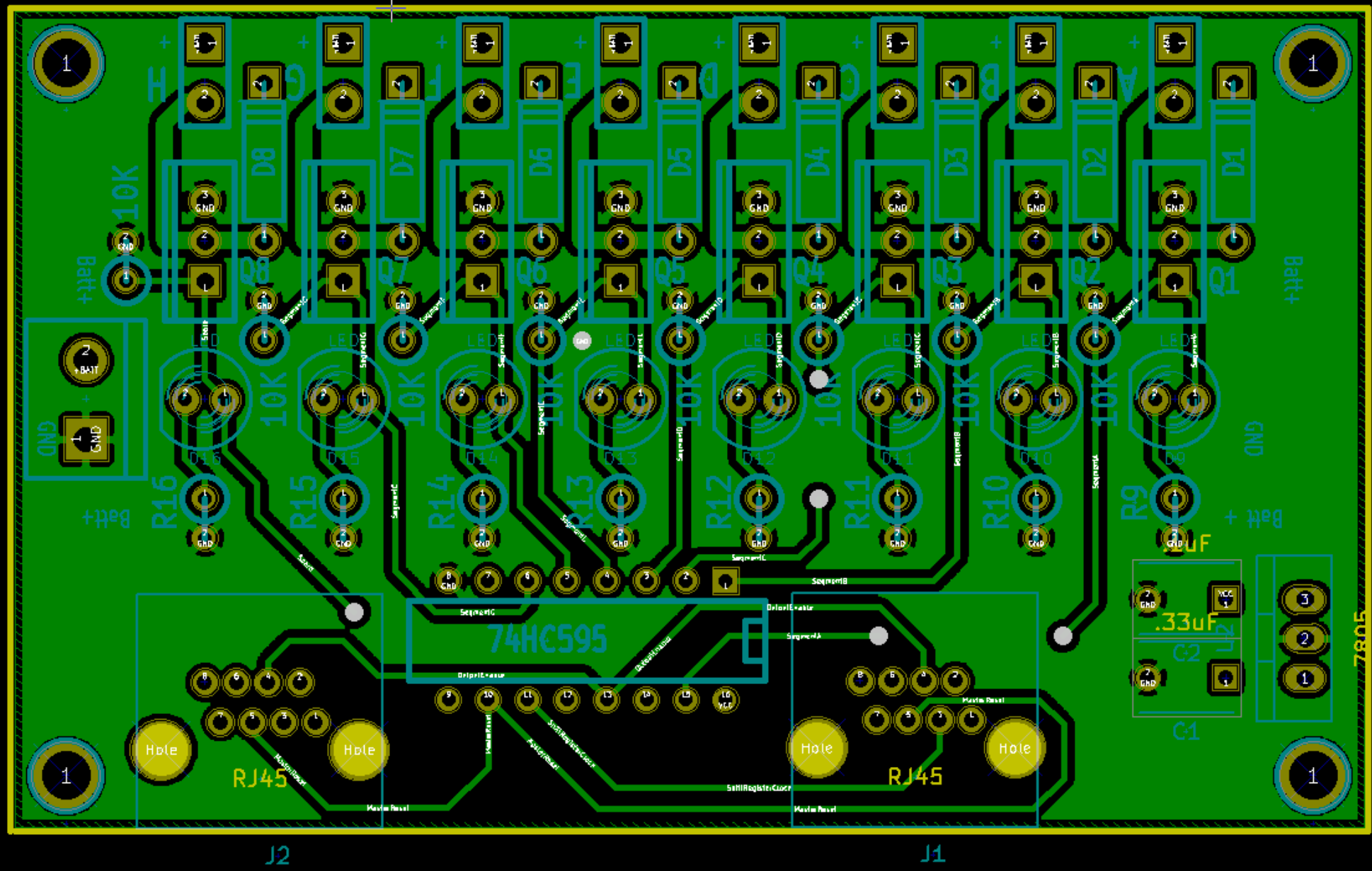
Copper (bottom) side traces only
