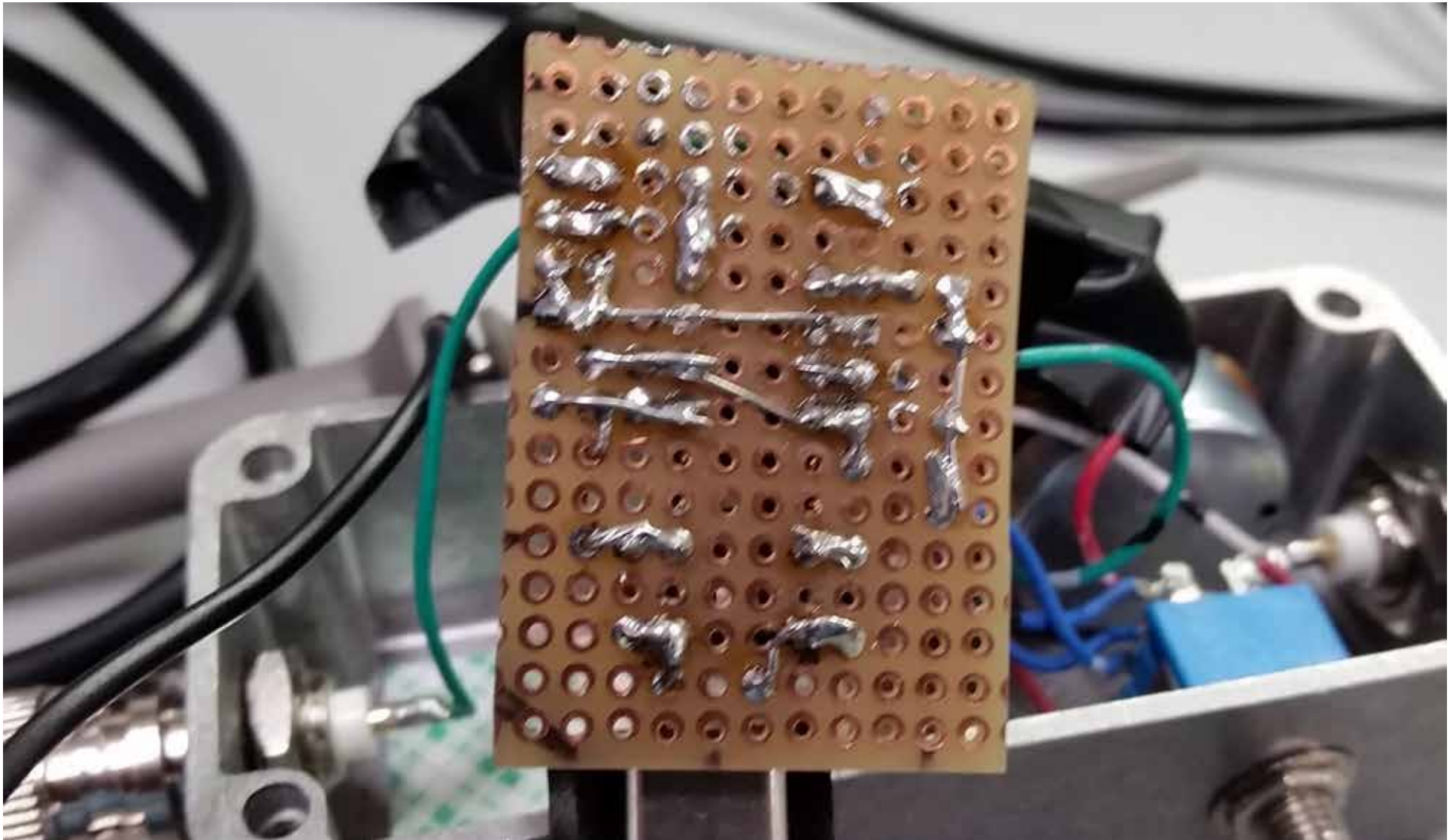
Copper Side of Circuit
