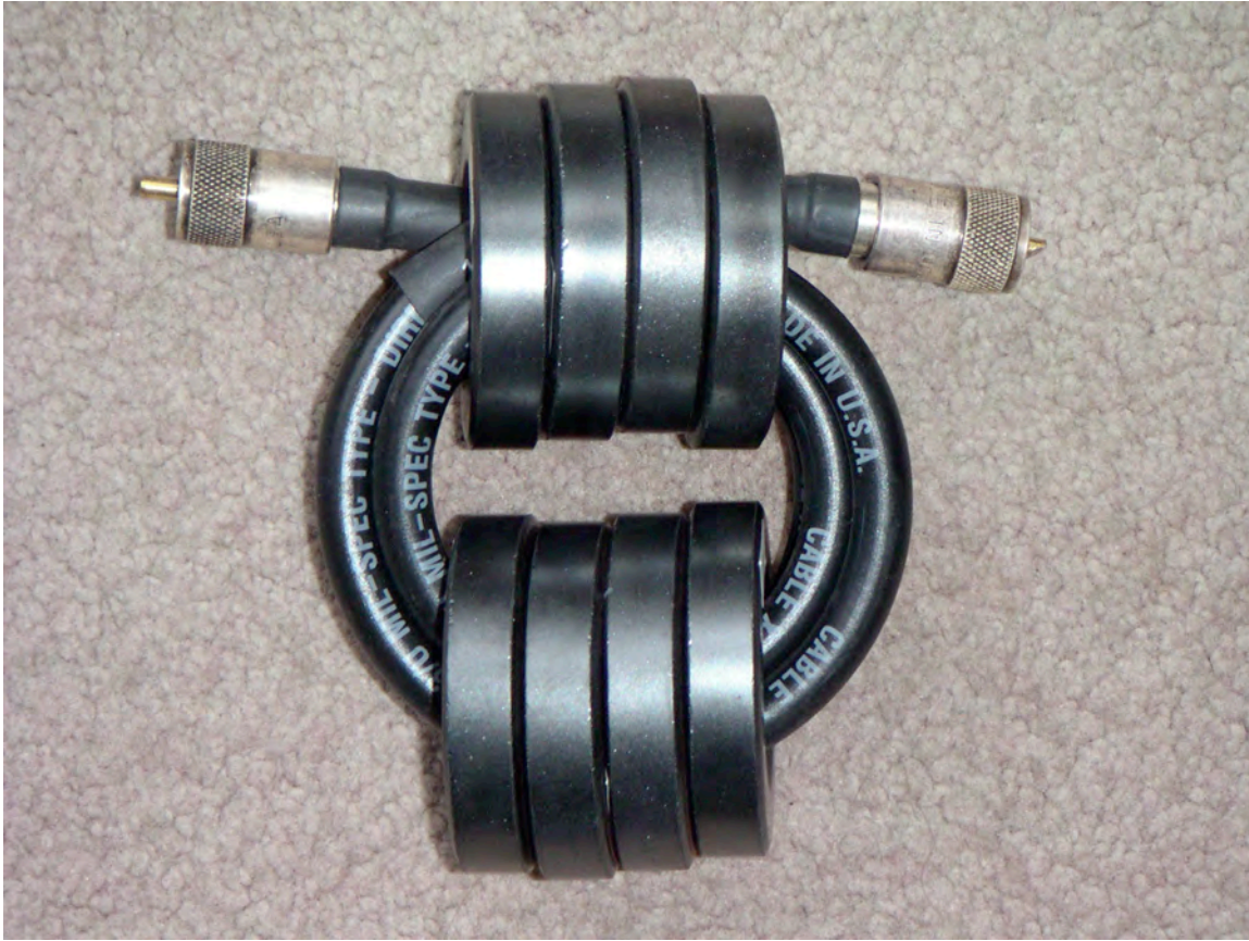
Figure 4: Common-mode choke for high HF power, formed by passing RG-213/U coaxial cable 3\frac{1}{2} times through a binocular core formed by two stacks of four Fair-Rite p/n 5943003801, mix-43, toroids. This choke's impedance exceeds 1\text{ k}\Omega from 1.8 through 18 MHz, dropping to 550\text{ }\Omega at 30 MHz. One such choke should be installed at the antenna feedpoint, one at the amplifier output, and at least one other in-between.
