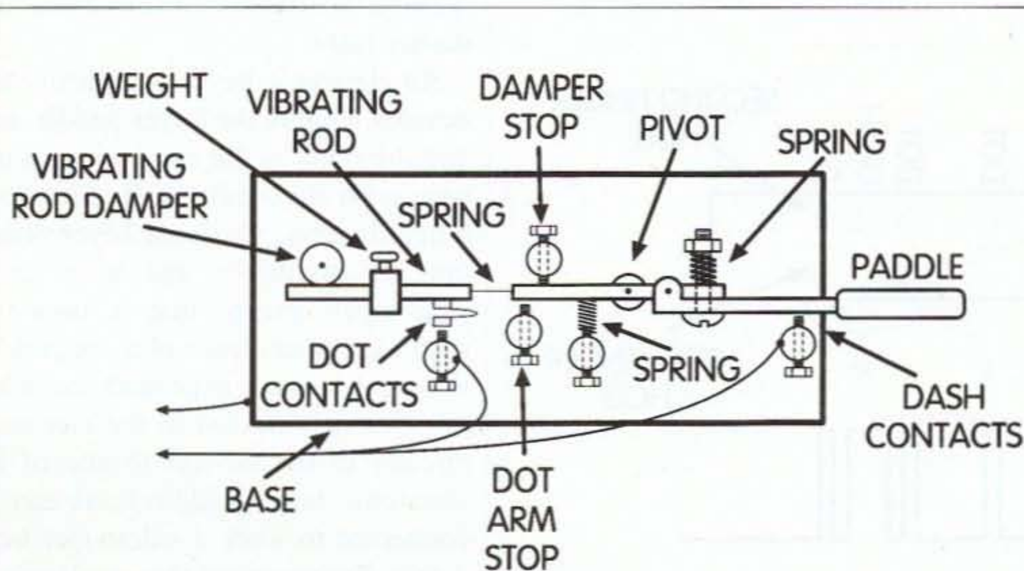
Fig. 3. Essentials of a semiautomatic key.
