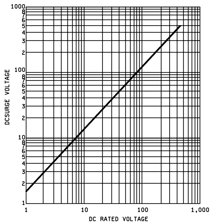
FIGURE 2. Surge voltage.
