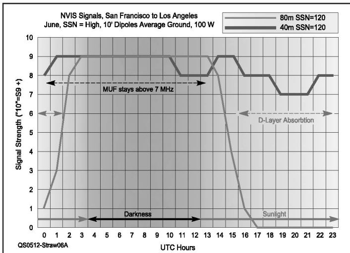
Figure 6—Signal strengths for the San Francisco to Los Angeles path for a worst-case month/SSN combination—summer solstice, in June, for a high level of solar activity (SSN = 120). Now 80 meters drops out more dramatically during the daylight hours, due to increased D-layer absorption. At this high level of solar activity, 40 meters remains open 24 hours with reasonable signal levels. However, the NVIS rule-of-thumb still holds: Use 40 meters during the day; 80 meters at night.
