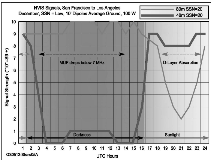
Figure 5—VOACAP calculations for a 350 mile path from San Francisco to Los Angeles, using 10 foot high flattop dipoles. This plot shows the signal strength in S Units ("S10" = S9+10) for a worst-case month/SSN combination—winter solstice, in December, for a low level of solar activity (SSN = 20). The 40 meter signal drops to a very low level during the night because the MUF drops well below 7.2 MHz. The 80 meter signal drops in the afternoon because of D-layer absorption. For 24 hour communications on this path, the rule of thumb is to select 40 meters during the day and 80 meters during the night.
