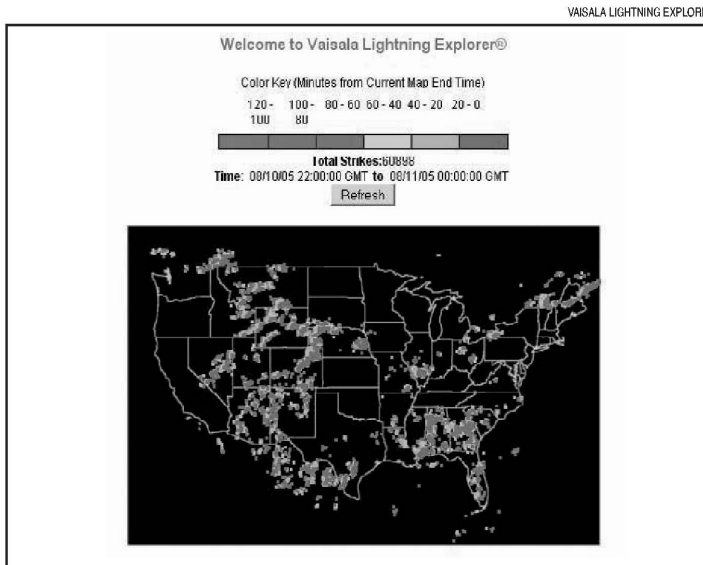
Figure 4—The distribution of lightning strikes across the USA for August 10, 2005 from 2200 to 0000 UTC, in the afternoon California time. There are lots of lightning strikes in the US during the summer—60,898 of them in this two-hour period!
