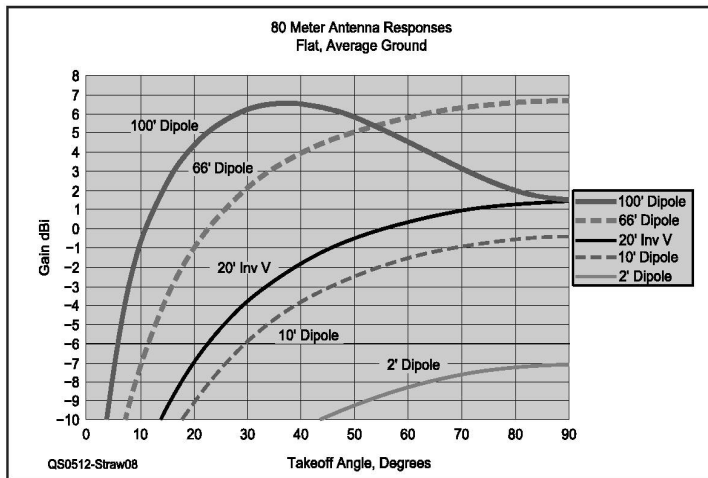
Figure 8—Elevation response patterns for 80 meter antennas over average soil. The shapes track each other rather well, remaining parallel for heights from 2 to 66 feet over flat ground. The 2 foot dipole is substantially down, about 9 dB, from the 20 foot Inverted V dipole at all angles.
