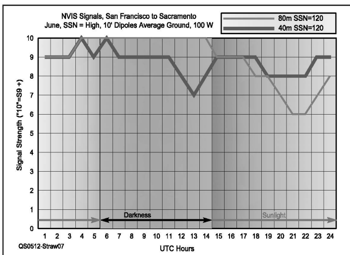
Figure 7—Signal strengths for a 75 mile path—San Francisco to Sacramento. This is for June and SSN = 120. Either band could be used successfully over the full 24 hour period because signal levels are always higher than S6. But the simple NVIS rule-of-thumb still holds: Use 40 meters during the day; 80 meters at night. This simplifies giving instructions to operators unaccustomed to the use of HF.
