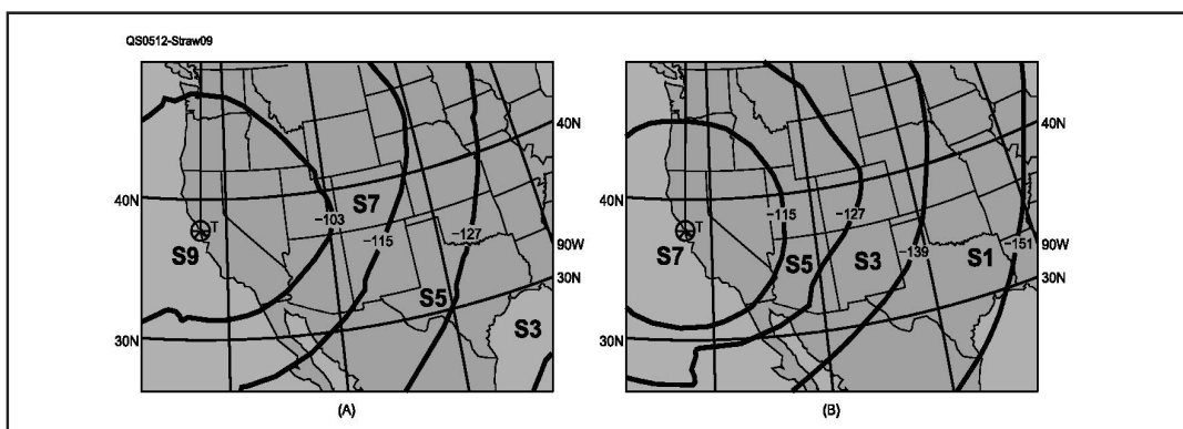
Figure 9—Geographic coverage plots for December, SSN = 20, 0300 UTC. At A, antennas are 20 foot high Inverted V dipoles over Average soil. At B, antennas are 2 foot high flattop dipoles over Average soil. The response for the 2 foot high antennas is down about 2 S units, 8 to 12 dB for a typical communications receiver.
