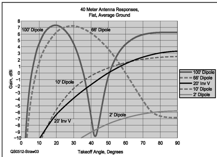
Figure 3—Elevation plots for different 40 meter antennas above flat ground with average ground characteristics (5 mS/m conductivity and dielectric constant of 13). The 10 foot high flattop dipole and the 20 foot high Inverted V dipoles both have close to the same characteristics. Note that there is a null in the response of the 100 foot high flattop dipole at a 42° elevation angle. The gain there is roughly that of a 2 foot high dipole!
